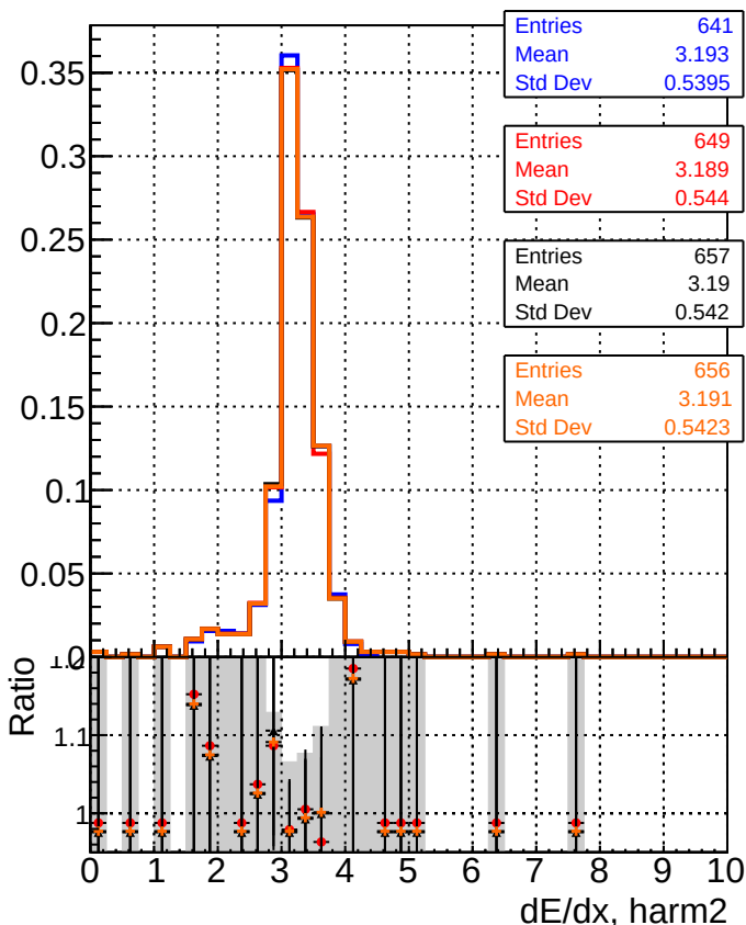
— DQM_mkFit_TToriginal — DQM_mkFit_TTNEW — DQM_mkFit_TTNEW50 — DQM_mkFit_TTNEW100
