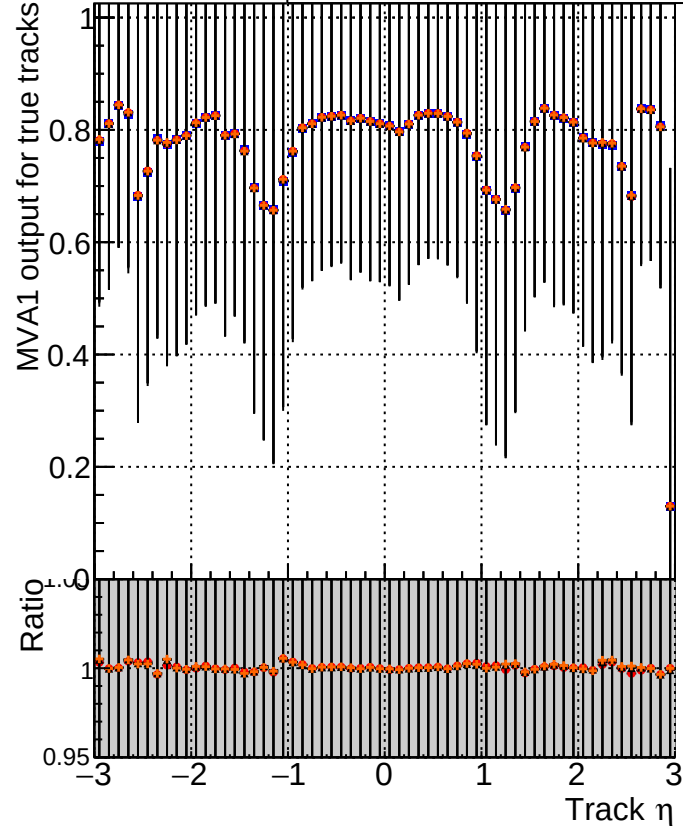
MVA1 of associated tracks (recoToSim) vs. track \eta Legend: \blacksquare DQM_mkFit_TToriginal \bullet DQM_mkFit_TTNEW \blacktriangledown DQM_mkFit_TTNEW50 \blacklozenge DQM_mkFit_TTNEW100
