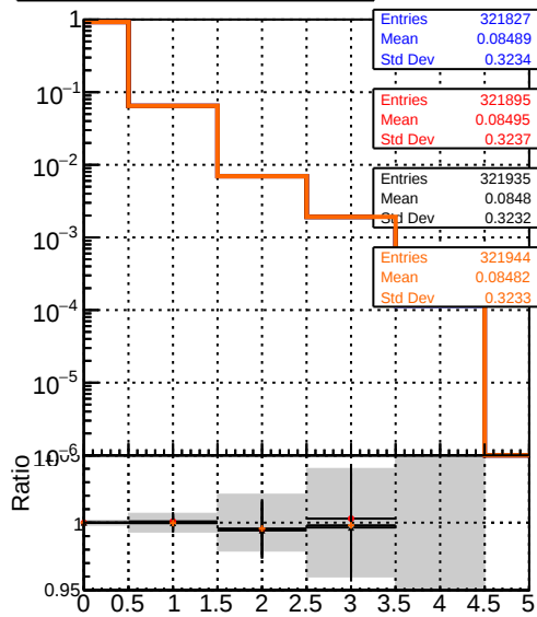
DQM_mkFit_TToriginal DQM_mkFit_TTNEW DQM_mkFit_TTNEW50 DQM_mkFit_TTNEW100 mean hit
