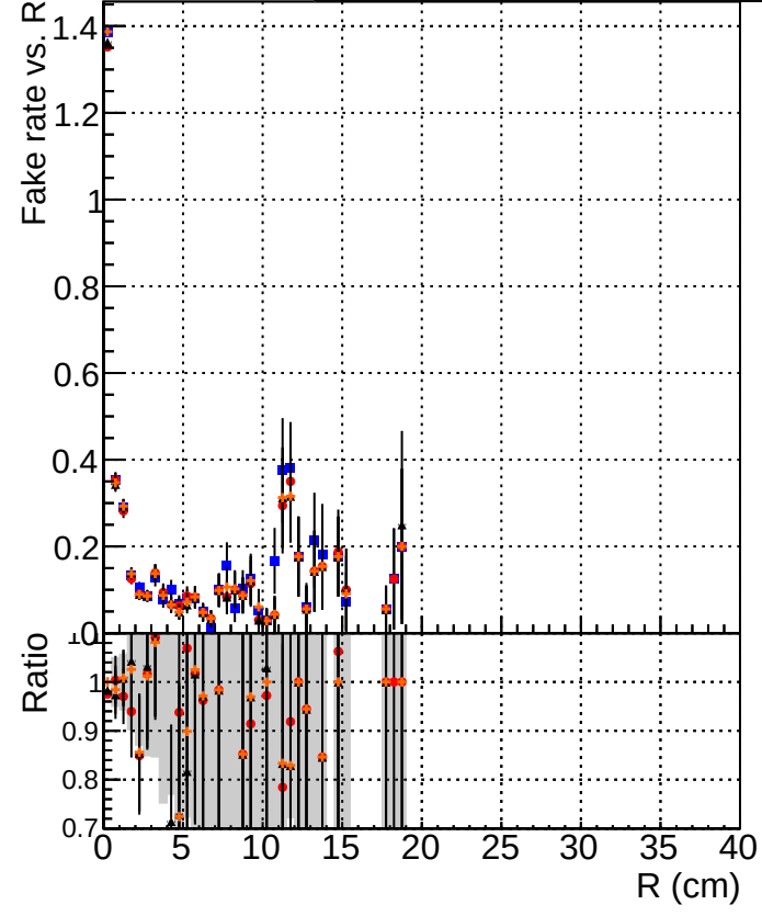
K_S^0 tracking fake rate vs R Legend: DQM_mkFit_TToriginal (blue square) DQM_mkFit_TTNEW (red circle) DQM_mkFit_TTNEW50 (black triangle) DQM_mkFit_TTNEW100 (orange star)
