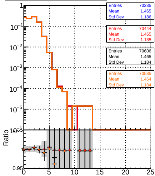
DQM_mkFit_TToriginal DQM_mkFit_TTNEW DQM_mkFit_TTNEW50 DQM_mkFit_TTNEW100 mean hits
