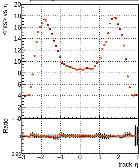
DQM_mkFit_TToriginal DQM_mkFit_TTNEW DQM_mkFit_TTNEW50 DQM_mkFit_TTNEW100 mean hit
