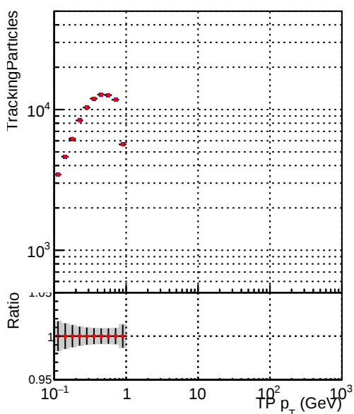
—•— DQM_V0001_R000000001_Global_CMSSW_original —•— DQM_V0001_R000000001_Global_CMSSW_cleaner
