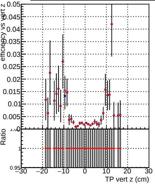
Efficiency vs TP vert z (cm) Legend: DQM_V0001_R000000001_Global_CMSSW_original DQM_V0001_R000000001_Global_CMSSW_cleaner
