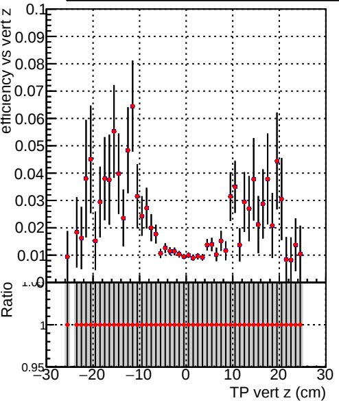
Efficiency vs vertpos Legend: DQM_V0001_R000000001_Global_CMSSW_original DQM_V0001_R000000001_Global_CMSSW_cleaner
