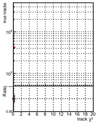
N of reco track vs. \chi^2 for DQM_V0001_R000000001_Global_CMSSW_original (black) and DQM_V0001_R000000001_Global_CMSSW_cleaner (red).
