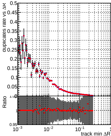
—■ DQM_V0001_R000000001_Global_CMSSW_original —◆ DQM_V0001_R000000001_Global_CMSSW_cleaner
