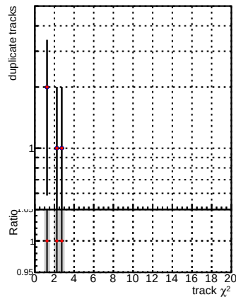
Legend: - \bullet DQM V0001_R000000001_Global_CMSSW_original - \bullet DQM V0001_R000000001_Global_CMSSW_cleaner - \bullet verSet
