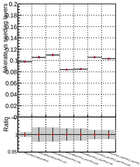
Fake rate vs. —●— DQM_V0001_R000000001 Global CMSSW_original —●— DQM_V0001_R000000001 Global CMSSW_cleaner
