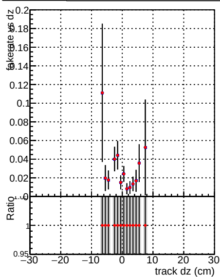
—●— DQM V0001_R000000001 Global CMSSW_original —●— DQM V0001_R000000001 Global CMSSW_cleaner
