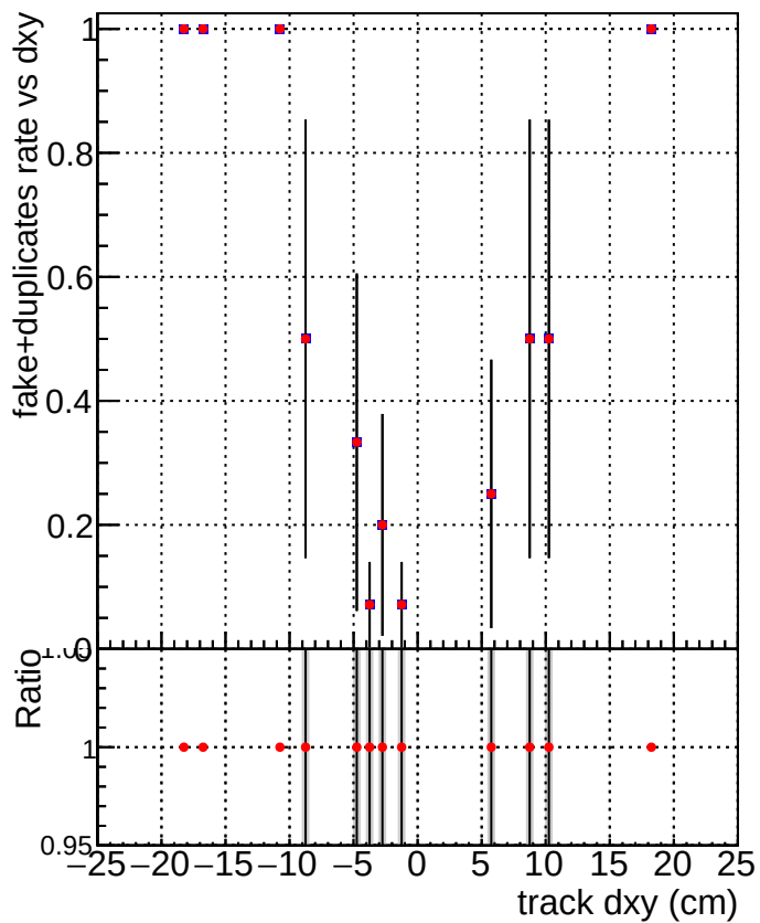
DQM_V0001_R000000001_Global_CMSSW_original DQM_V0001_R000000001_Global_CMSSW_cleaner
