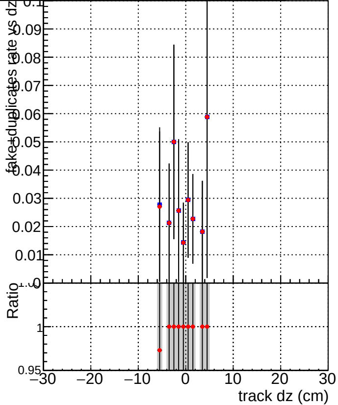
DQM_V0001_R000000001_Global_CMSSW_original DQM_V0001_R000000001_Global_CMSSW_cleaner
