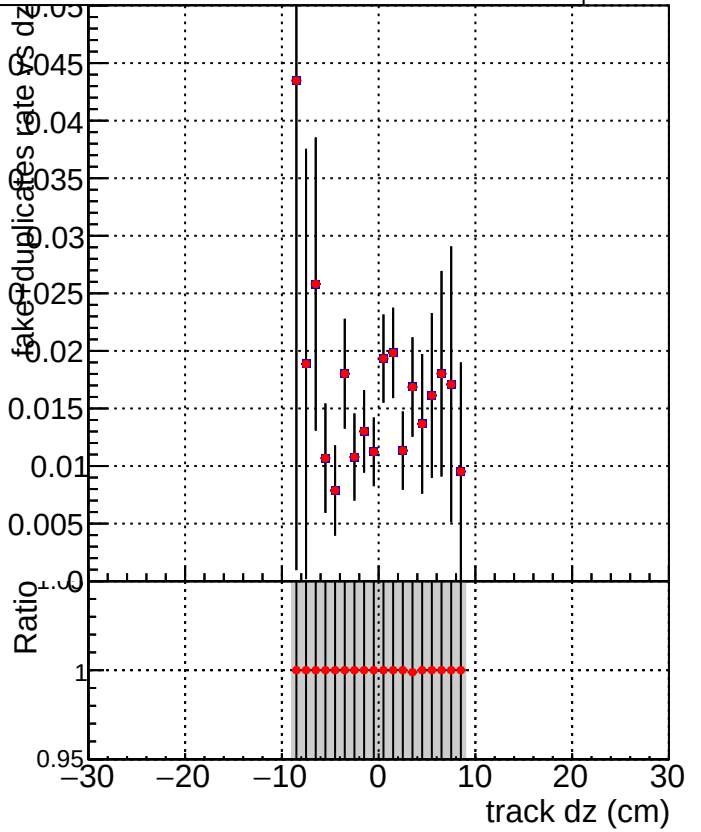
DQM_V0001_R000000001_Global_CMSSW_original DQM_V0001_R000000001_Global_CMSSW_cleaner
