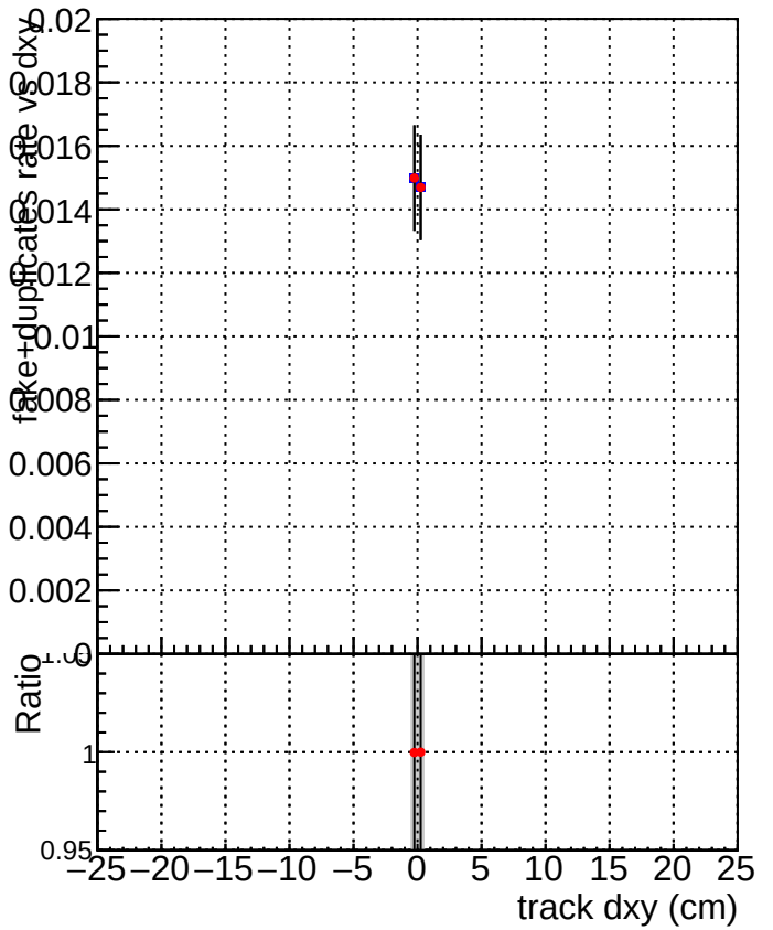
DQM_V0001_R000000001_Global_CMSSW_original DQM_V0001_R000000001_Global_CMSSW_cleaner
