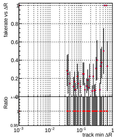
—●— DQM_V0001_R000000001_Global_CMSSW_original —●— DQM_V0001_R000000001_Global_CMSSW_cleaner
