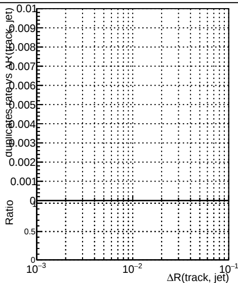
—●— DQM_V0001_R000000001_Global_CMSSW_original —●— DQM_V0001_R000000001_Global_CMSSW_cleaner
