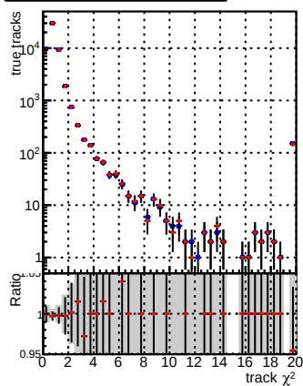
N of reco track vs. \chi^2 Legend: DOM_V0001_R000000001_Global_CMSSW_original DOM_V0001_R000000001_Global_CMSSW_cleaner
