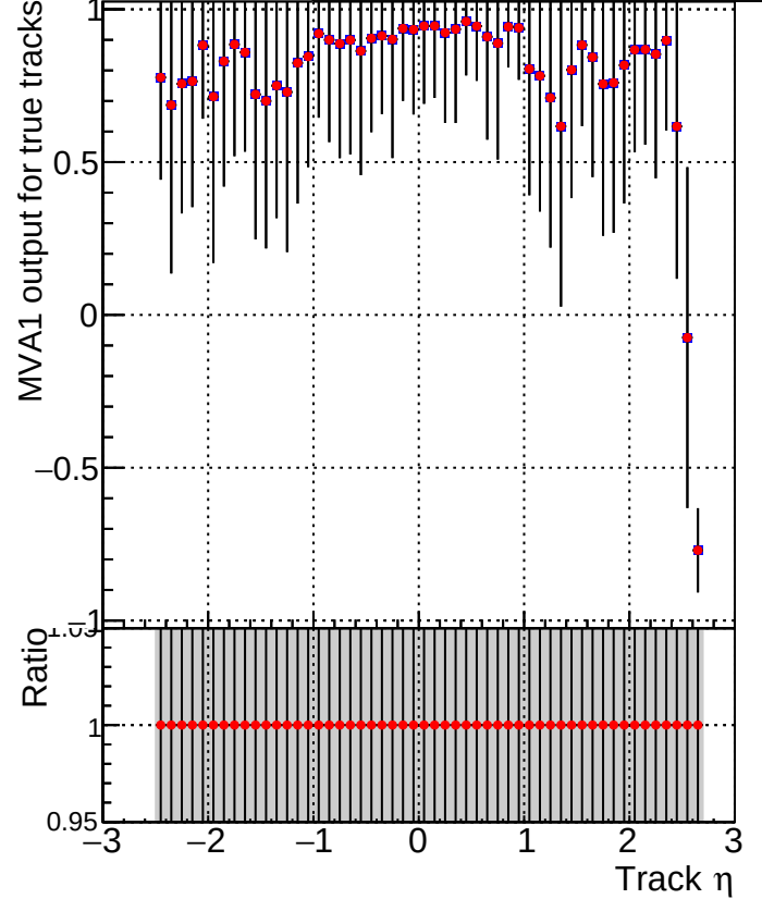
MVA1 of associated tracks (recoToSim) vs. track \eta Legend: ■ DQM_V0001_R000000001_Global_CMSSW_original ■ DQM_V0001_R000000001_Global_CMSSW_cleaner
