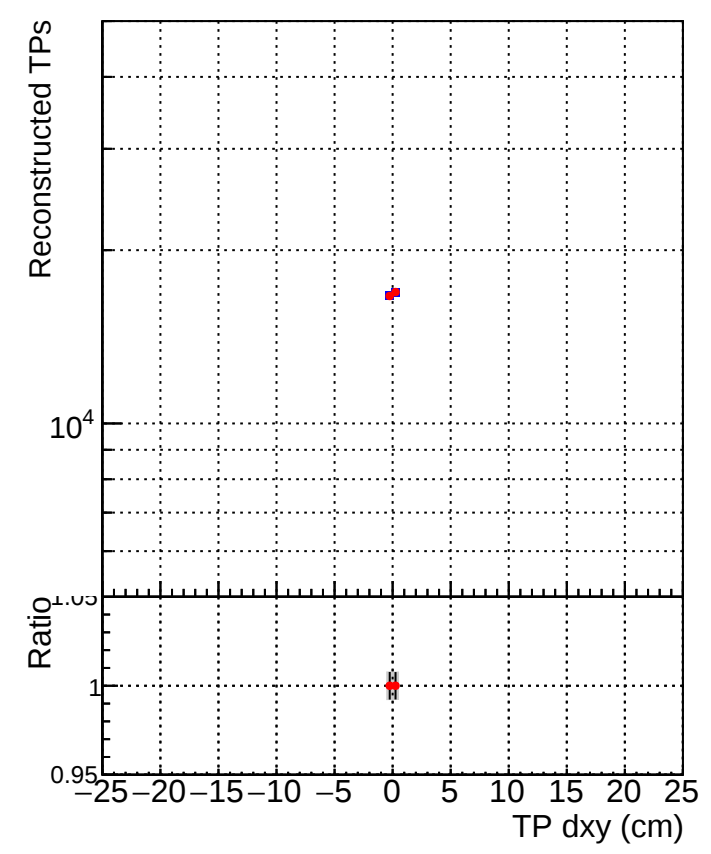
N of simulated track DQM_V0001_R000000001_Global_CMSSW_original DQM_V0001_R000000001_Global_CMSSW_cleaner
