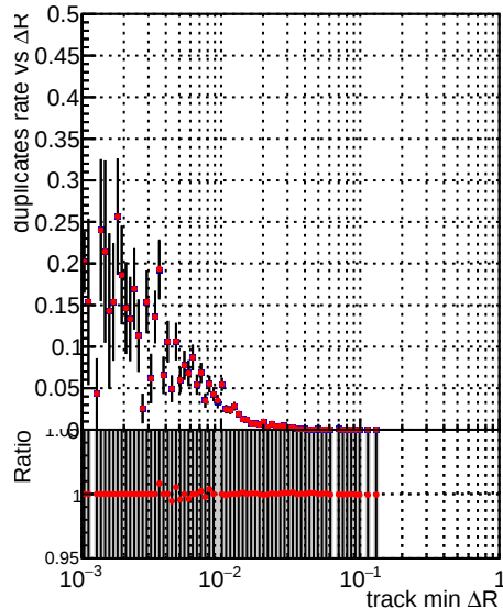
—•— DQM_V0001_R000000001_Global_CMSSW_original —•— DQM_V0001_R000000001_Global_CMSSW_cleaner
