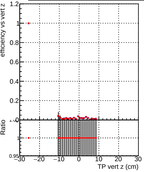
Efficiency vs vert z Legend: DQM_V0001_R000000001_Global_CMSSW_original DQM_V0001_R000000001_Global_CMSSW_cleaner
