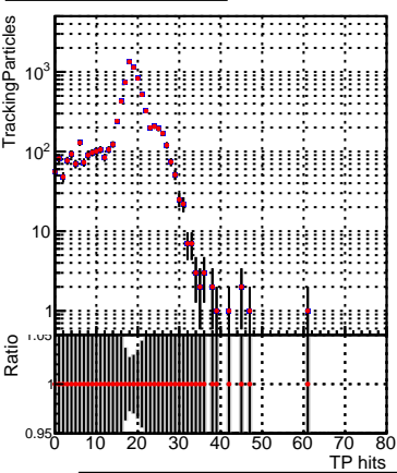
■ DQM_V0001_R000000001_Global_CMSSW_original ■ DQM_V0001_R000000001_Global_CMSSW_cleaner
