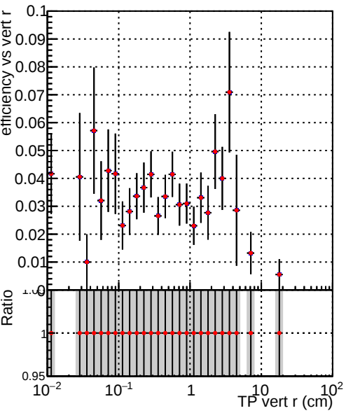
Efficiency vs TP vert r (cm) Legend: DQM_V0001_R000000001_Global_CMSSW_original DQM_V0001_R000000001_Global_CMSSW_cleaner
