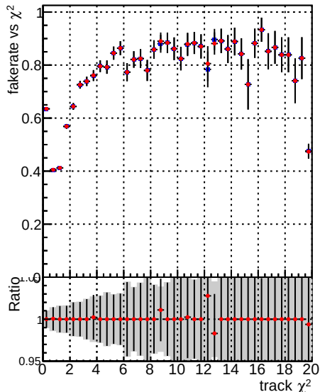
Fake rate vs. Legend Global CMSSW Blue square DQM V0001_R000000001 original Red circle DQM V0001_R000000001 cleaner
