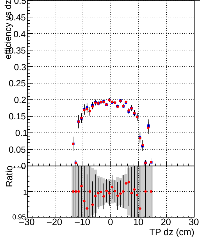
Efficiency vs Dz Legend: DQM_mkFit_TToriginal (Blue squares) DQM_mkFit_TTNEWHWS_ALLITERS (Red circles)
