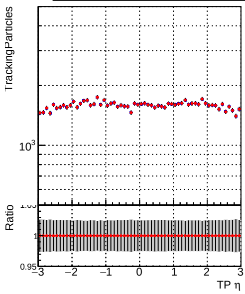
N of simulated tracks vs \eta Legend: DQM_mkFit_TToriginal (blue line), DQM_mkFit_TTNEWSH_ALLITERS (red line)
