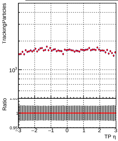
Legend: DQM_mkFit_TToriginal (blue line), DQM_mkFit_TTNEWSH_ALLITERS (red line)
