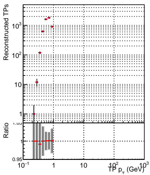
Legend: \blacksquare DQM_mkFit_TToriginal \bullet DQM_mkFit_TTNEWHs_ALLITERS
