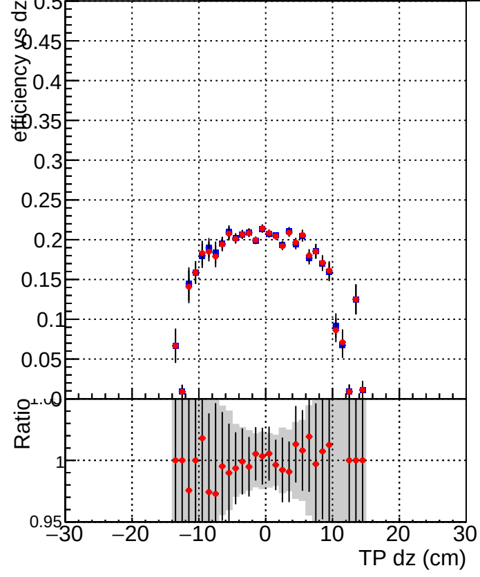
Efficiency vs Dz Legend: DQM_mkFit_TToriginal (Blue square) DQM_mkFit_TTNEWHWS_ALLITERS (Red circle)
