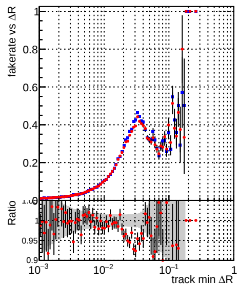
—●— DQM_mkFit_TToriginal —●— DQM_mkFit_TTNEWHS_ALLITERS
