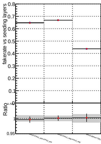
Fake rate vs. —•— DQM_mkFit_TToriginal —•— DQM_mkFit_TTNEWHS_ALLITERS
