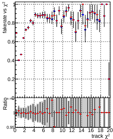
Fake rate vs. —•— DQM_mkFit_TToriginal —•— DQM_mkFit_TTNEWHS_ALLITERS
