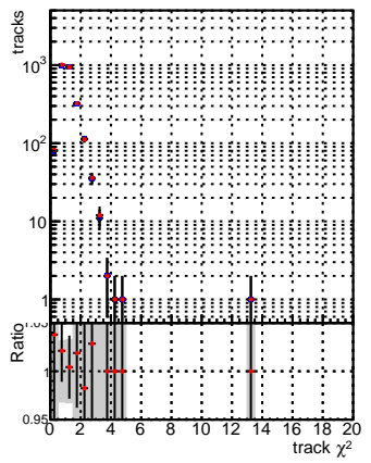
N of reco track vs. \chi^2 —•— DQM_mkFit_TToriginal —•— DQM_mkFit_TTNEWS ALLITERS
