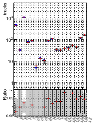
N of reco track vs. \chi^2 —•— DQM_mkFit_TToriginal —•— DQM_mkFit_TTNEWS ALLITERS
