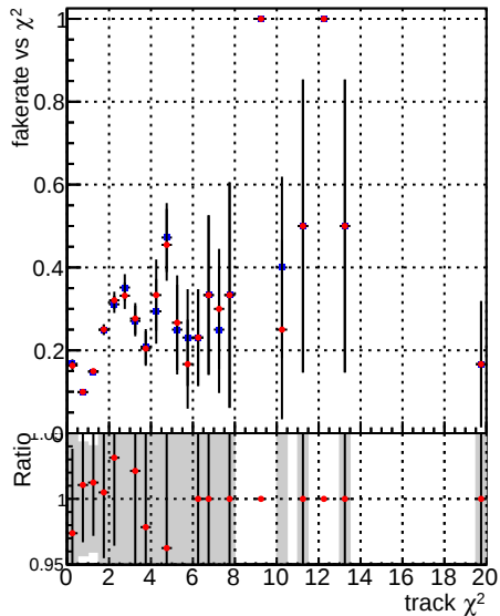
Fake rate vs. \chi^2 —•— DQM_mkFit_TToriginal —•— DQM_mkFit_TTNEWS ALLITERS
