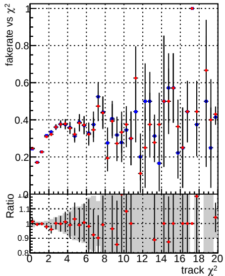
Fake rate vs. —•— DQM_mkFit_TToriginal —•— DQM_mkFit_TTNEWS ALLITERS
