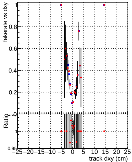
—●— DQM_mkFit_TToriginal —●— DQM_mkFit_TTNEWSH_ALLITERS
