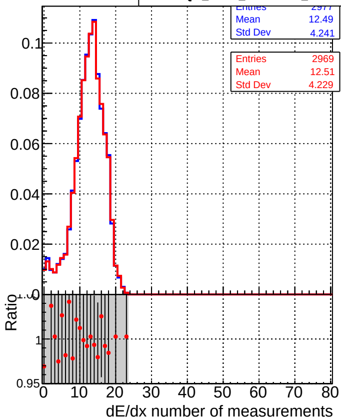
—■— DQM_mkFit_TToriginal —●— DQM_mkFit_TTNEWSH_ALLITERS
