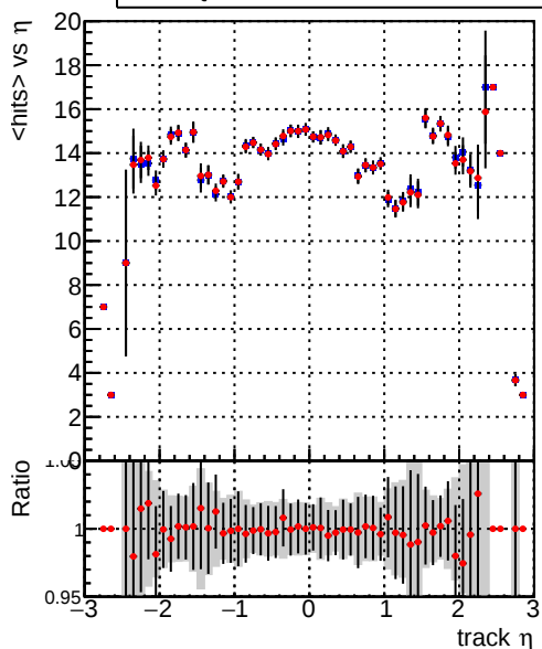
mean hit — DQM_mkFit_TToriginal — DQM_mkFit_TTNEWHS_ALLITERS
