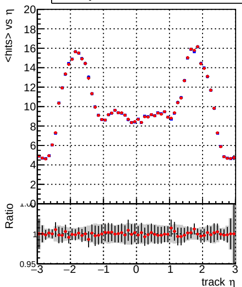
mean hit — DQM_mkFit_TToriginal — DQM_mkFit_TTNEWHS_ALLITERS
