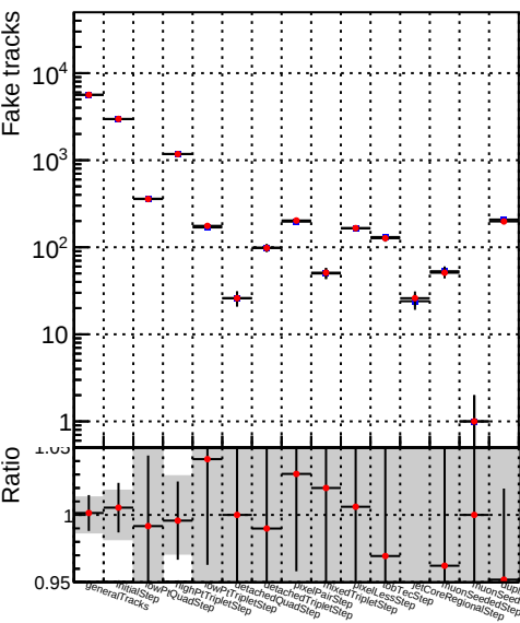
Number —●— DQM_mkFit_TTNEWHS_ALLITERS
