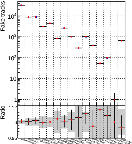
Number —●— DQM_mkFit_TTNEWHS_ALLITERS
