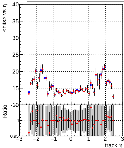
mean hits vs \eta Legend: DQM_mkFit_TToriginal (blue line), DQM_mkFit_TTNEWHS_ALLITERS (red line)
