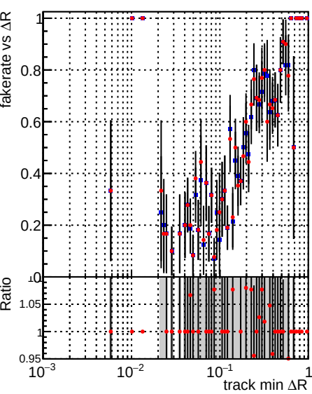
Fake rate vs \Delta R (track, jet) DQM_mkFit_TToriginal DQM_mkFit_TTNEWHS_ALLITERS
