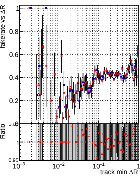
Legend: DQM_mkFit_TToriginal (blue squares), DQM_mkFit_TTNEWHS_ALLITERS (red circles)
