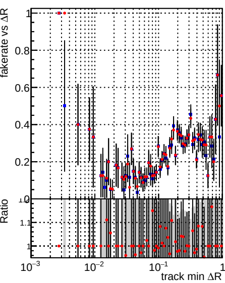
Fake rate vs \Delta R(\text{track, jet}) Legend: DQM_mkFit_TToriginal (blue), DQM_mkFit_TTNEWHS_ALLITERS (red)
