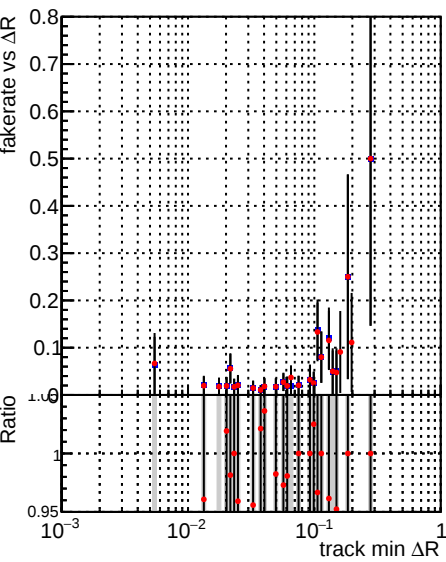
Fake rate vs \Delta R(\text{track, jet}) Legend: DQM_mkFit_TToriginal (grey squares), DQM_mkFit_TTNEWHS_ALLITERS (red circles)
