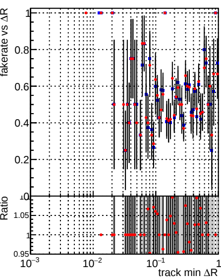
Fake rate vs \Delta R(\text{track, jet}) Legend: DQM_mkFit_TToriginal (blue dots), DQM_mkFit_TTNEWHS_ALLITERS (red dots)
