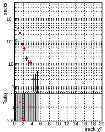
Legend: DQM_mkFit_TToriginal (blue line with circles), DQM_mkFit_TTNEWHS_ALLITERS (red line with circles)
