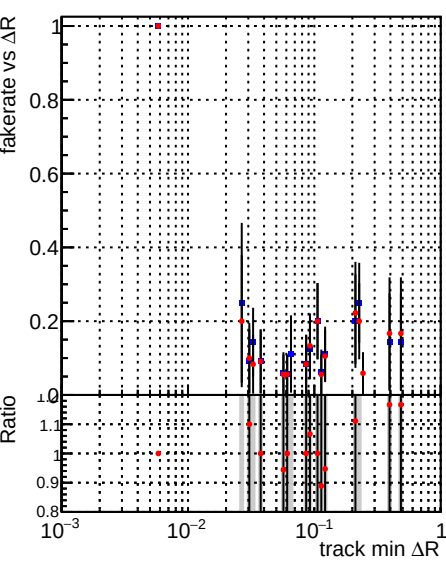
Fake rate vs \Delta R(\text{track, jet}) DQM_mkFit_TToriginal DQM_mkFit_TTNEWHS_ALLITERS
