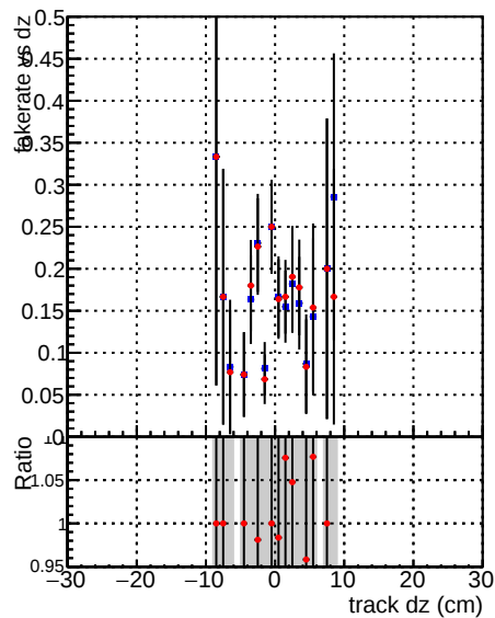
—•— DQM_mkFit_TToriginal —•— DQM_mkFit_TTNEWHS_ALLITERS
