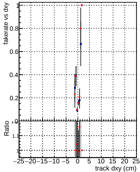
—•— DQM_mkFit_TToriginal —•— DQM_mkFit_TTNEWHS_ALLITERS
